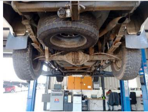
undercarriage rear.
