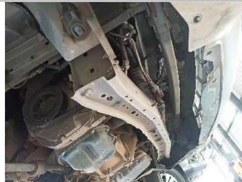
Radiator Cradle
