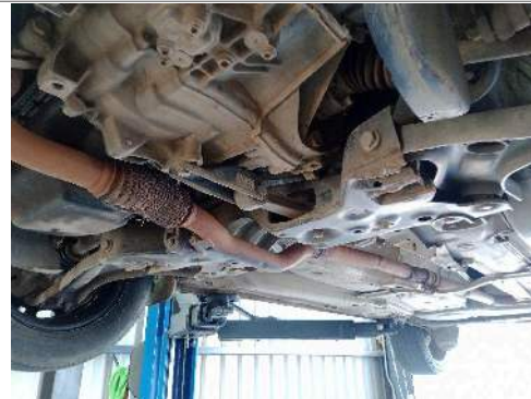
Sub Frame
