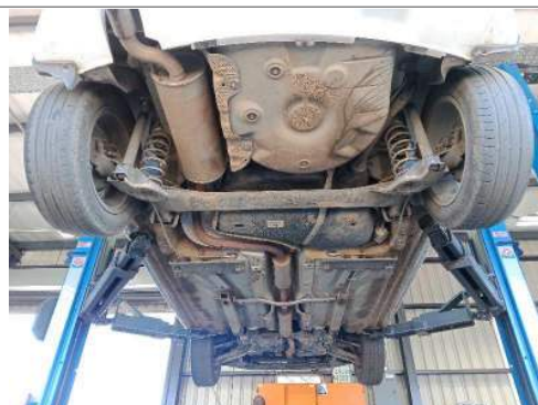
Rear end
